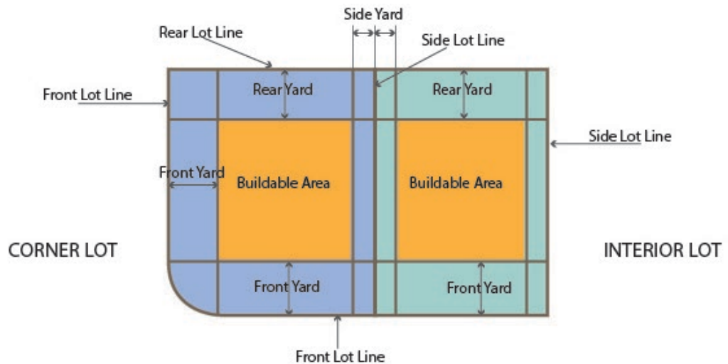
Figure 5.5 | Yard Setbacks
