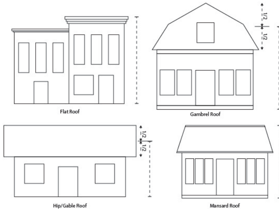
Figure 5.3 | Building Height Measurements
